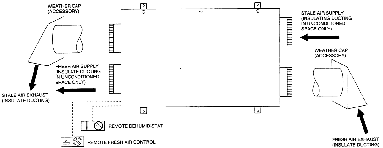
Fig. 4—Typical system components for ER200.
