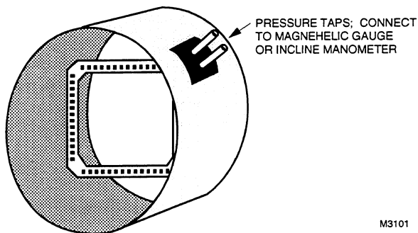
Fig. 16—Airflow measurement grid.
