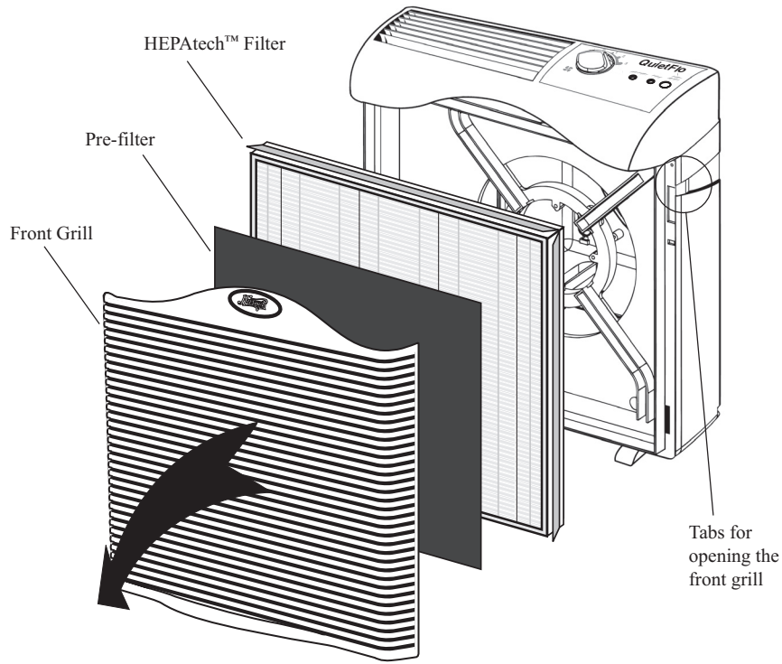
Figure 1 - Model 30240
