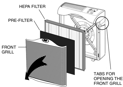
Fig. 2 - Air Purifier Components
