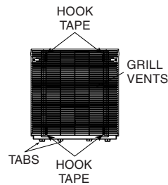
Fig. 3 - Inside Surface of Front Grill
