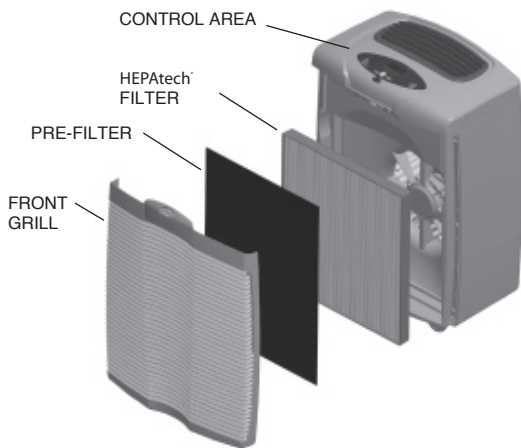
Fig. 2 - Air Purifier Components
