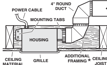
HOUSING MOUNTED TO ADDITIONAL FRAMING Discharge 90° to joists.
