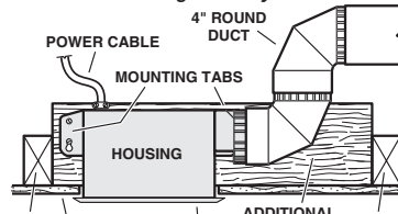
HOUSING MOUNTED TO 2x4 TRUSS Requires additional framing for mounting tabs. Discharge 90° to joists.
