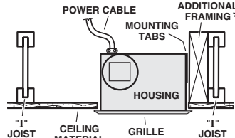
HOUSING MOUNTED TO "1" JOIST Requires additional framing for mounting tabs. Discharge parallel to joists.
