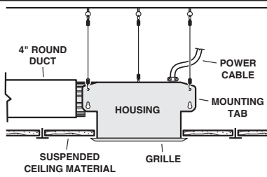
SUSPENDED CEILINGS Housing hung with wires - 3-point mount. INSTALL THE HOUSING
