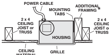
HOUSING MOUNTED TO 2x4 TRUSS Requires additional framing for mounting tabs. Discharge parallel to joists.
