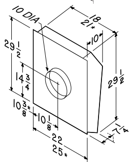
Models 335 & 336 Exterior Blowers
