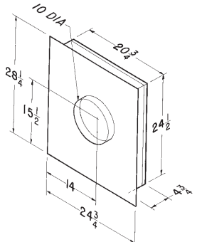
Models 331H & 332H Exterior Blowers
