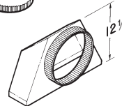
Model 424 4½ x 18½ to 10" Rd. Front/Rear Transition
