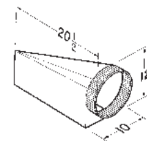
Model 453 4½ x 18½ to 10" Rd. Left Transition (shown)
