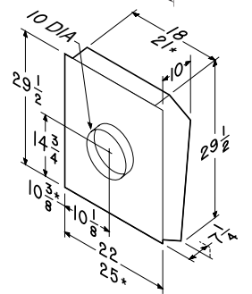
Models 335 & 336 Exterior Blowers
