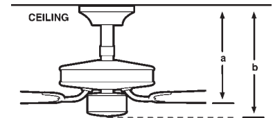
Standard Downrod Mount
