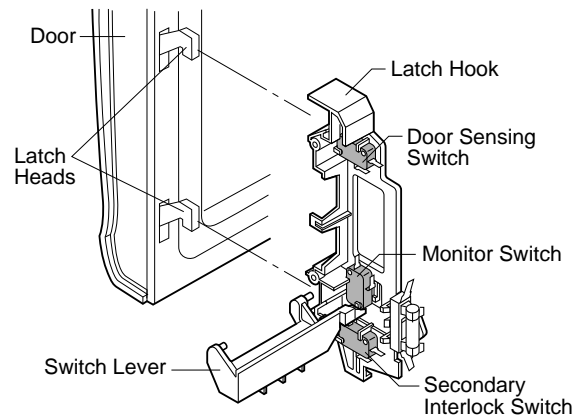
Figure C-3. Latch Switch Adjustments
