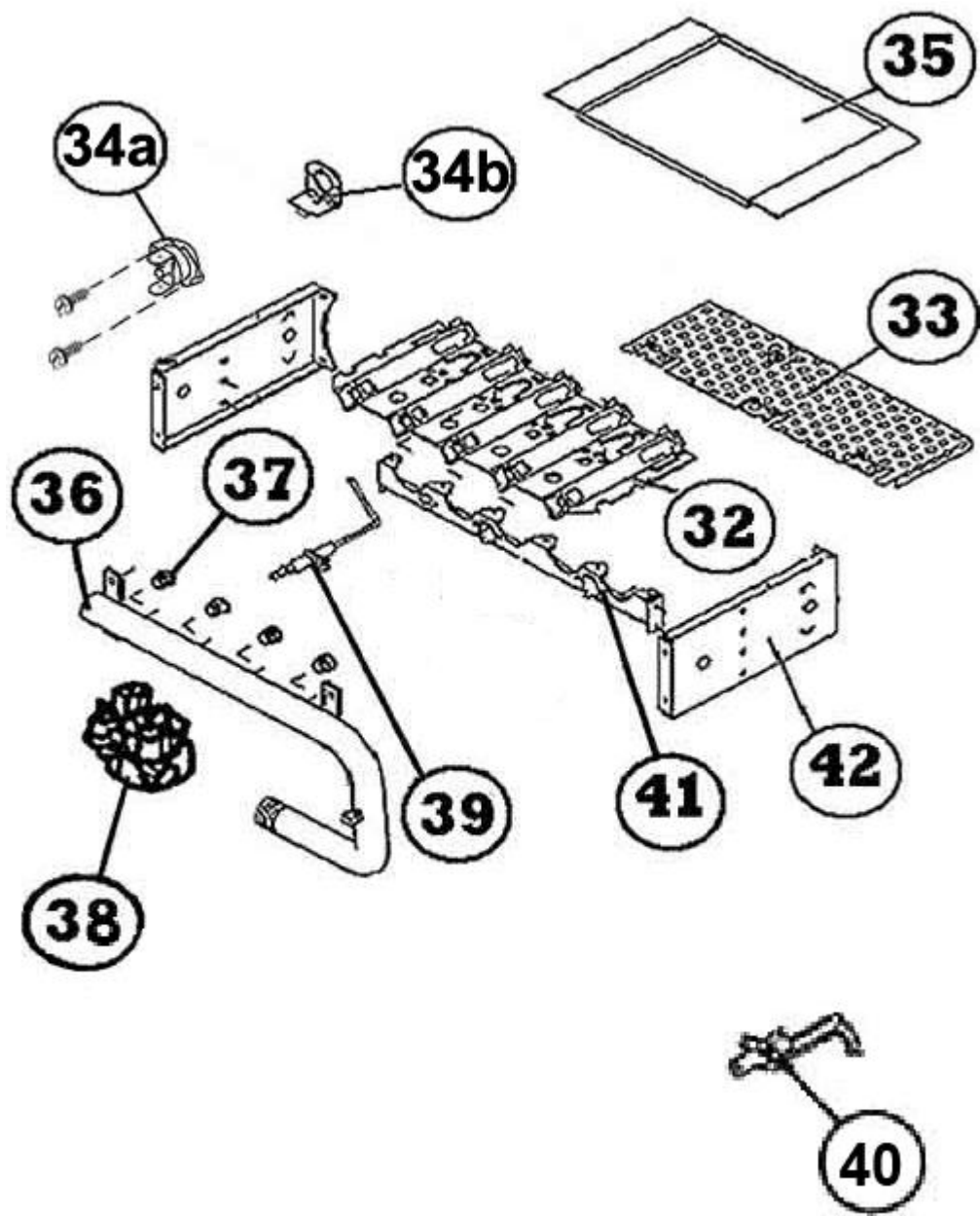
Burner Assembly
