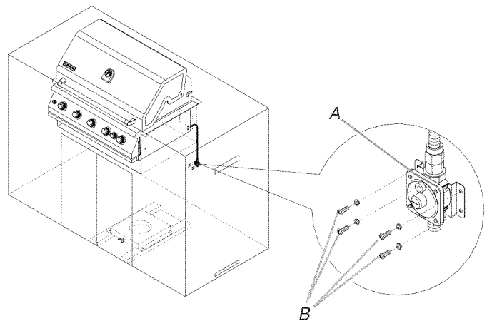
A. Natural gas pressure regulator B. Four 1/2" x 10 mm truss head screws
