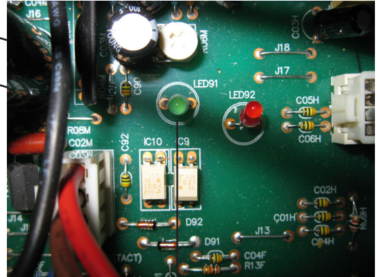
Location of PCB LED: To access, remove outdoor unit cover, and then remove lid to PCB box.
