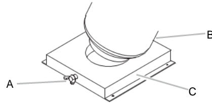
A. Locking screw B. Tank tray C. 20 lb LP gas fuel tank tray
