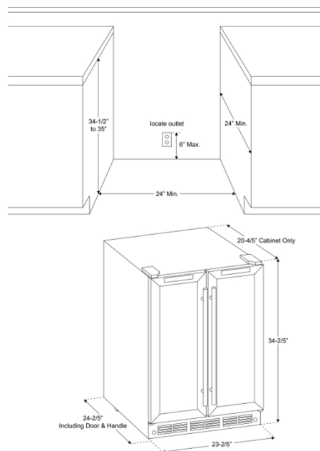
Figure A – The cutout depth must be 24"
