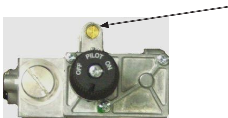
Figure 4.3 Pilot Adjustment Screw
