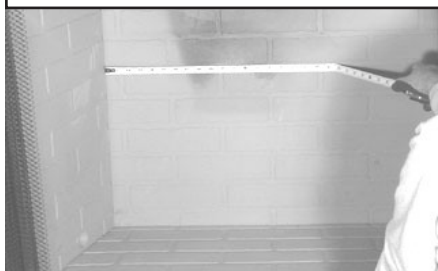
Figure 2.1 Measure Firebox
