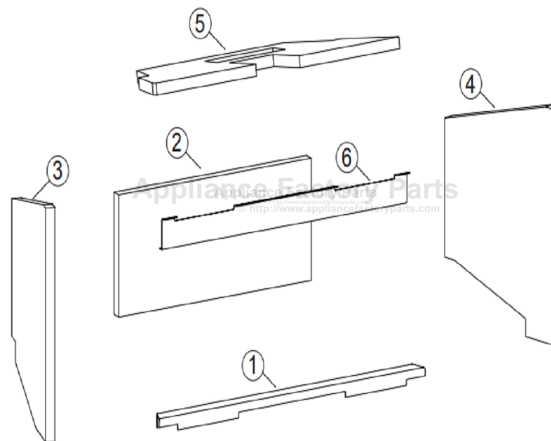
CERAMIC FIBER LINER KIT EXPLODED VIEW AND PARTS LIST
