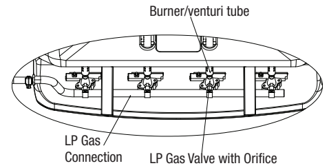
Figure 1: Main Burners
