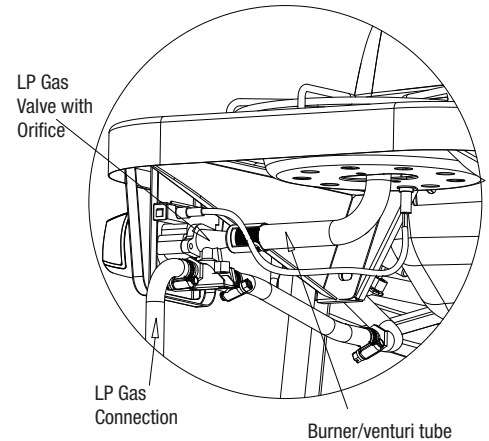
Figure 2: Side Burner
